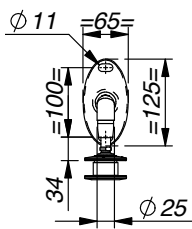
BOTTOM BRACKET
