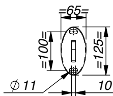
TOP BRACKET
