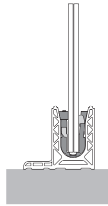
OFFSET MOUNTING
