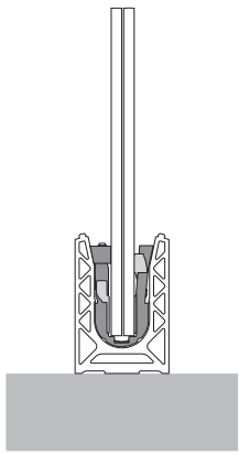
FLOOR MOUNTING
