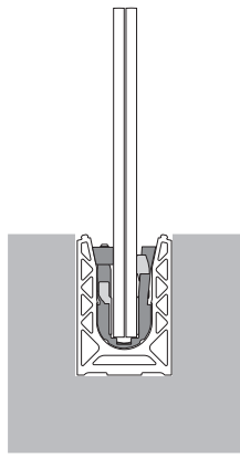
BUILT-IN-SLAB
