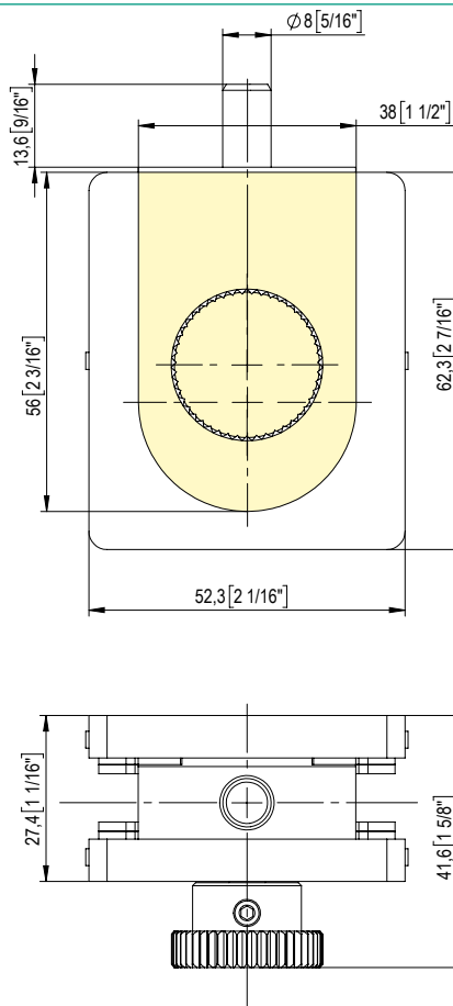
BOCCOLA INCLUSA - FLOOR BUSHING INCLUDED
