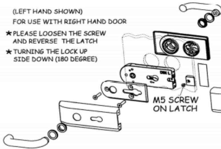
LK-500SBL (Long Strike Box)
