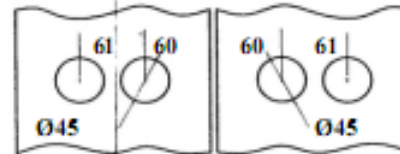
SIZE OF GLASS CUTOUT W/ Long Strike Box (LK-500 & LK-500SBL)
