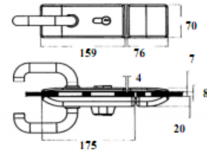
GLASS DOOR TO SIDE FIXED PANEL
