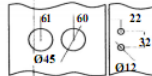
SIZE OF GLASS CUTOUT W/ Long Strike Box (LK-500 & LK-500SBL)
